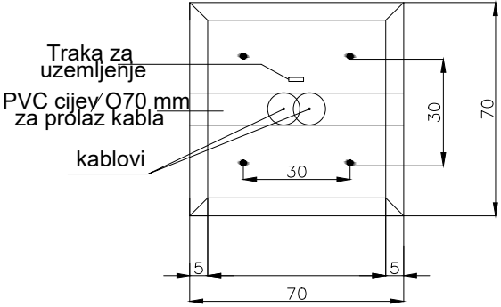
RASPORED ANKERA
