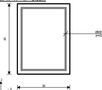
Presek 47-47 x = 0.00m
