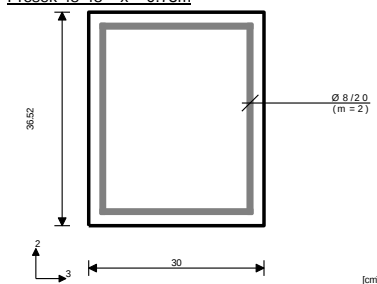
Presek 48-48 x = 0.73m
