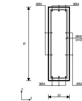
Presek 5-5 x = 0.85m
