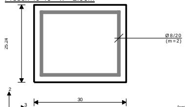
Presek 40-40 x = 2.96m
