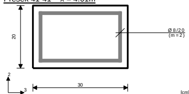
Presek 41-41 x = 4.01m
