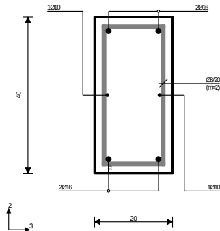
Presek 34-34 x = 0.86m
