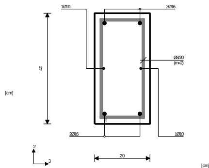
Presek 39-39 x = 4.31m
