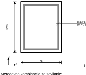
Presek 21-21 x = 0.45m
