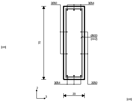
Presek 8-8 x = 4.23m
