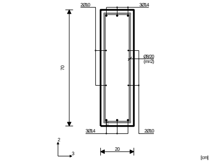
Presek 9-9 x = 0.00m
