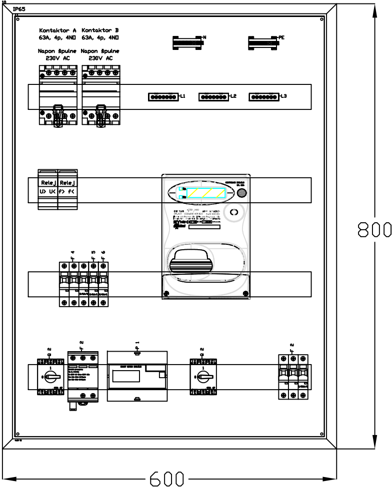
Ormar RO-P-S2
