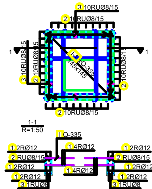
PLAN ARMATURE
